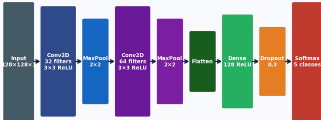
Fig. 4. Proposed CNN Architecture for Engine Fault Classification.
